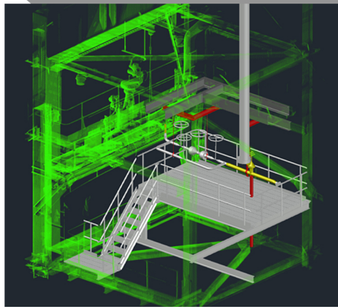
3D LASER SCAN POINT CLOUD & 3D MODEL OF ACCESS PLATFORMS
