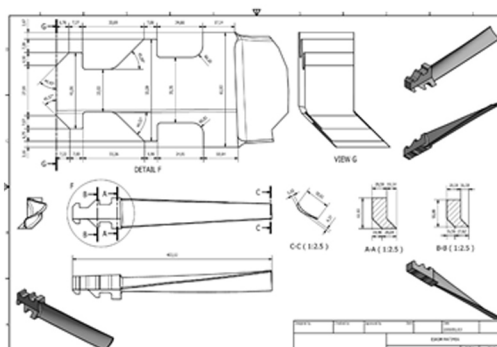
REVERSE ENGINEERING & DETAIL DRAWINGS
